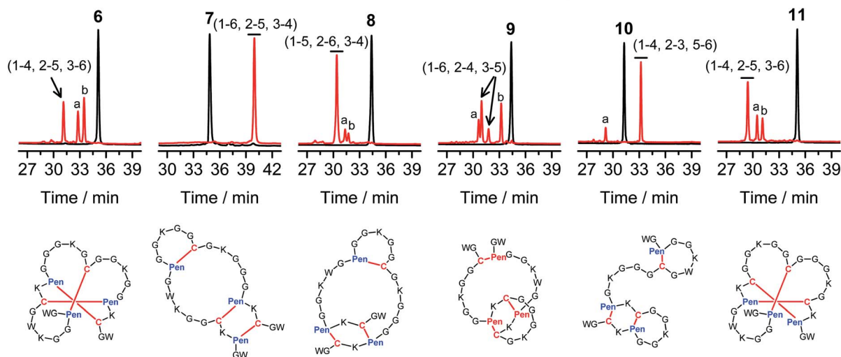
Fig. 3 Amino acid sequences of peptides 6–11 (from N- to C-terminus). Chromatograms showing the oxidation of 6–11 (10 μM) in 0.2 mM GSSG (100 mM phosphate buffer, pH 7.4) (black line: before oxidation; red line: 2 h after oxidative folding). Topological drawings of the expected folds were given in bottom panels (red lines denote disulfide bonds; amino acid sequences can be read in a counter-clockwise direction). The disulfide connectivity of peaks a and b shown in the chromatograms (by products): 6-a = (1-6, 2-5, 3-4), 6-b = (1-4, 2-3, 5-6); 8-a = (1-5, 2-6, 3-4), 8-b = (1-4, 2-6, 3-5); 9-a = (1-5, 2-4, 3-6), 9-b = (1-2, 3-5, 4-6); 10-a = (1-6, 2-3, 4-5); 11-a = (1-4, 2-6, 3-5), 11-b = (1-3, 2-5, 4-6). Disulfide pairings were established by tryptic digestion HPLC and mass spectrometry (Fig. S15–S36†). Of note, a pair of conformers formed from the folding of 9, which have identical disulfide connectivity (1-6, 2-4, 3-5).
