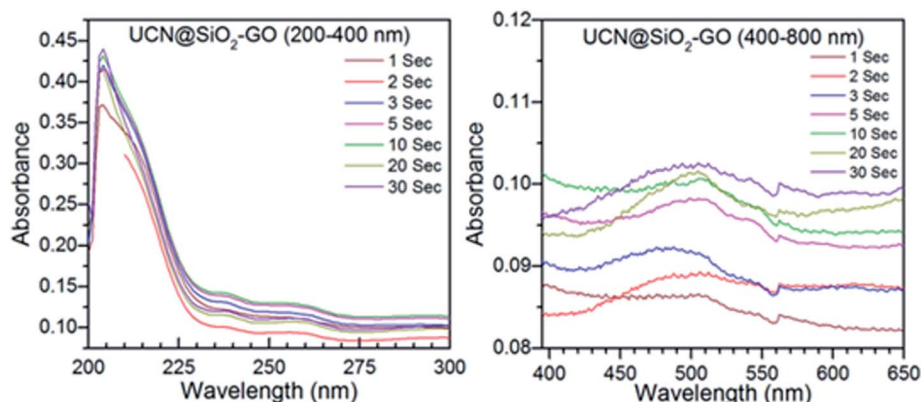
Fig. 10 Time dependent release of DOX studied through UV-Visible absorption spectra for UCN@SiO 2 -GO nanocomposite.
