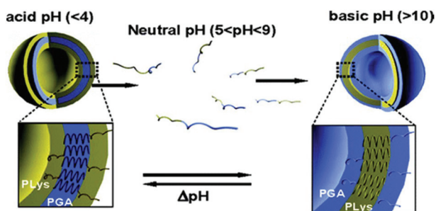
Fig. 3 Schematic representation of pH-regulated schizophrenic vesicles from the self-assembly of the diblock copolypeptide PGA 15 -b-PLys 15 in water. Reprinted with permission from ref. 15. Copyright (2005) American Chemical Society.
