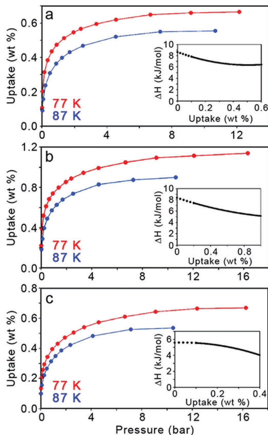
Fig. 14 (top) Bottom-up synthesis of heteroatom-substituted carbons; reaction conditions: tetraglyme, diphenyl ether, or paraffin oil solvent, X = halogen or OR, and temperatures between 250 and 350 °C. (bottom) Hydrogen uptake at 77 and 87 K for (a) boron-, (b) phosphorus-, and (c) nitrogen-substituted carbons. Adapted with permission from Z. Jin, Z. Z. Sun, L. J. Simpson, K. J. O'Neill, P. A. Parilla, Y. Li, N. P. Stadie, C. C. Ahn, C. Kittrell and J. M. Tour, J. Am. Chem. Soc. , 2010, 132 , 15246. Copyright 2008 American Chemical Society.
