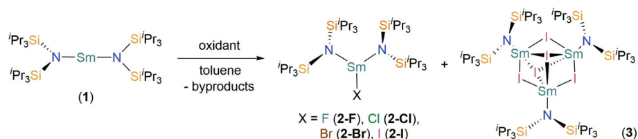
Scheme 1 Synthesis of [Sm(N †† ) 2 (X)] (X = F, 2-F ; Cl, 2-Cl ; Br, 2-Br ; I, 2-I ) and [Sm(N †† ) 3 (μ 2 -I) 3 (μ 3 -I) 2 ] ( 3 ) by the treatment of [Sm(N †† ) 2 ] ( 1 ) with various oxidants; 2-F : +[Fe(Cp) 2 ][PF 6 ], –[Fe(Cp) 2 ], and PF 5 ; 2-Cl , 2-Br : + t BuX, –CH 3 CH(CH 3 )CH 3 , and –CH 2 =C(CH 3 )CH 3 ; 2-I , 3 : +0.5 I 2 and –unidentified by-products.
