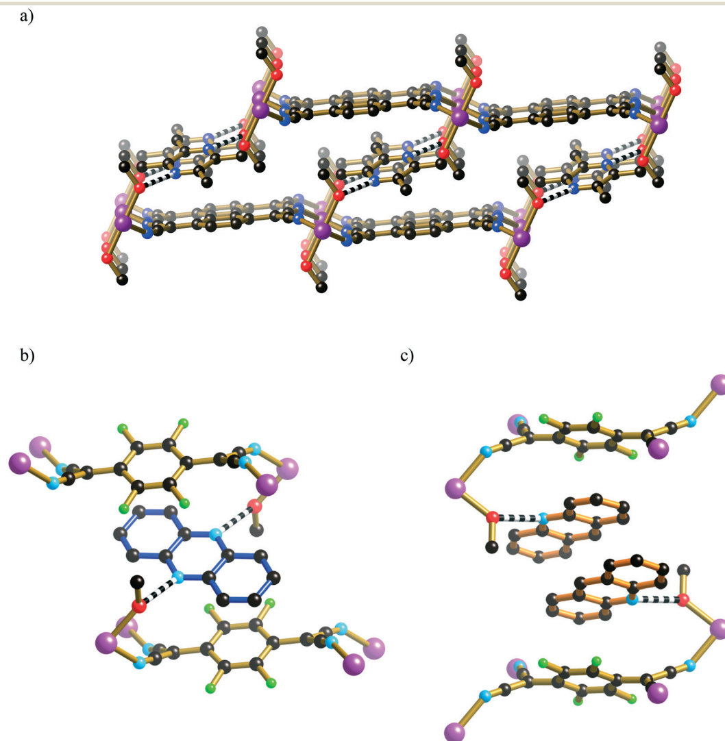
Fig. 3 a) The structure of [Zn(TCNQ)(MeOH) 2 ].tmpyz ( 14 ) in which sheets are linked via H-bonding between coordinated MeOH ligands and tetra-methylpyrazine units (H-bonds represented by striped connections). b) The structure of [Mn(F 4 TCNQ)(MeOH) 2 ].phenazine ( 16 ) showing the H-bonding and aromatic interactions of the phenazine molecule. c) The H-bonding and stacking in [Mn(F 4 TCNQ)(MeOH) 2 ].2acridine ( 17 ).
