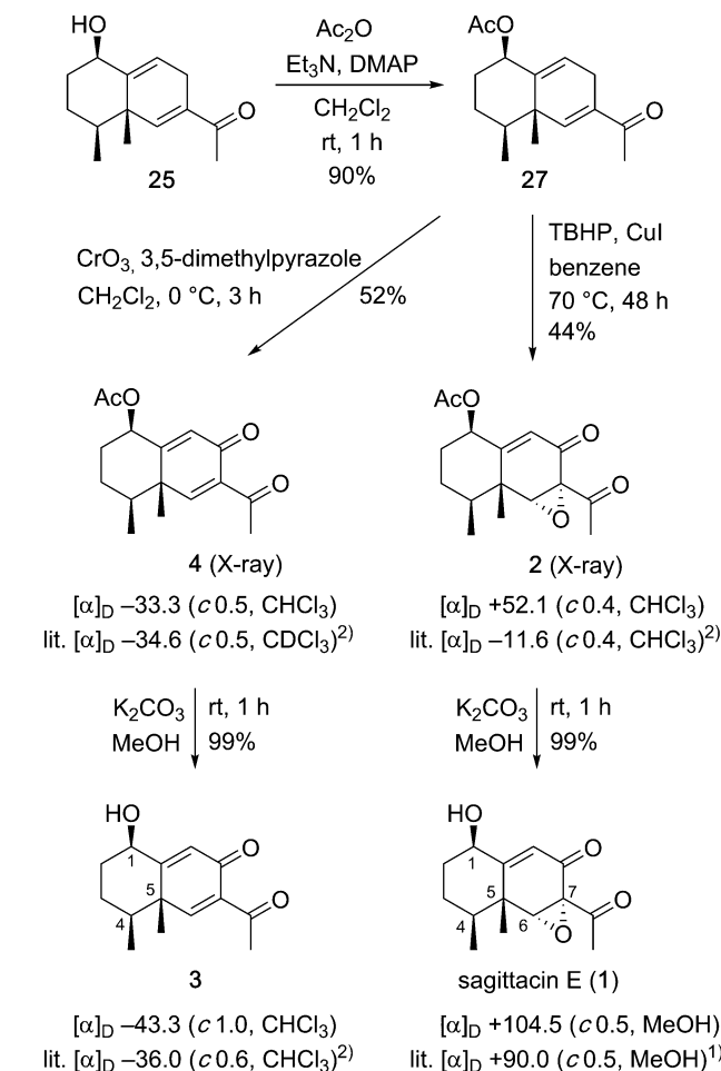
Scheme 5 Asymmetric synthesis of sagittacin E ( 1 ) and related natural products.
