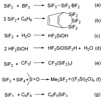
Scheme 1 The reactions of a SiF 4 -SiF 2 mixture with various substrates.
