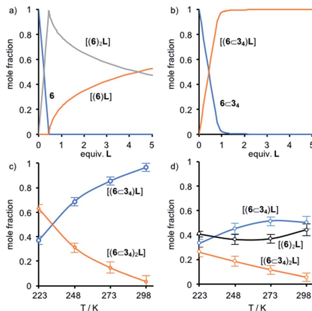
Fig. 4 Speciation diagrams for (a) 6 with respect to equiv. L ; (b) 6C34 with respect to equiv. L ; (c) L in a 6C34 + 0.4 L mixture with respect to T ; (d) L in a 6 + 6C34 + L (1 : 1 : 1) mixture with respect to T .
