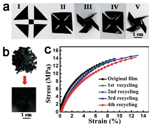
Fig. 2 Heat responses of ACAT–vitrimers due to the intrinsic malleable property of vitrimers. (a) Welding (I–II) at temperature above T_v (200 °C, oven), permanent reshaping (II–III) at temperatures above T_v (200 °C, oven), temporary reshaping (III and IV) above T_g but below T_v (80 °C, oven) and shape memory (IV and V) by reheating above T_g (80 °C, oven). The thickness of the vitrimer films used here was about 0.2 mm. (b) Demonstration of the recycling process (with a thickness of about 0.2 mm). (c) Stress–strain curves for the recycled and original films.
