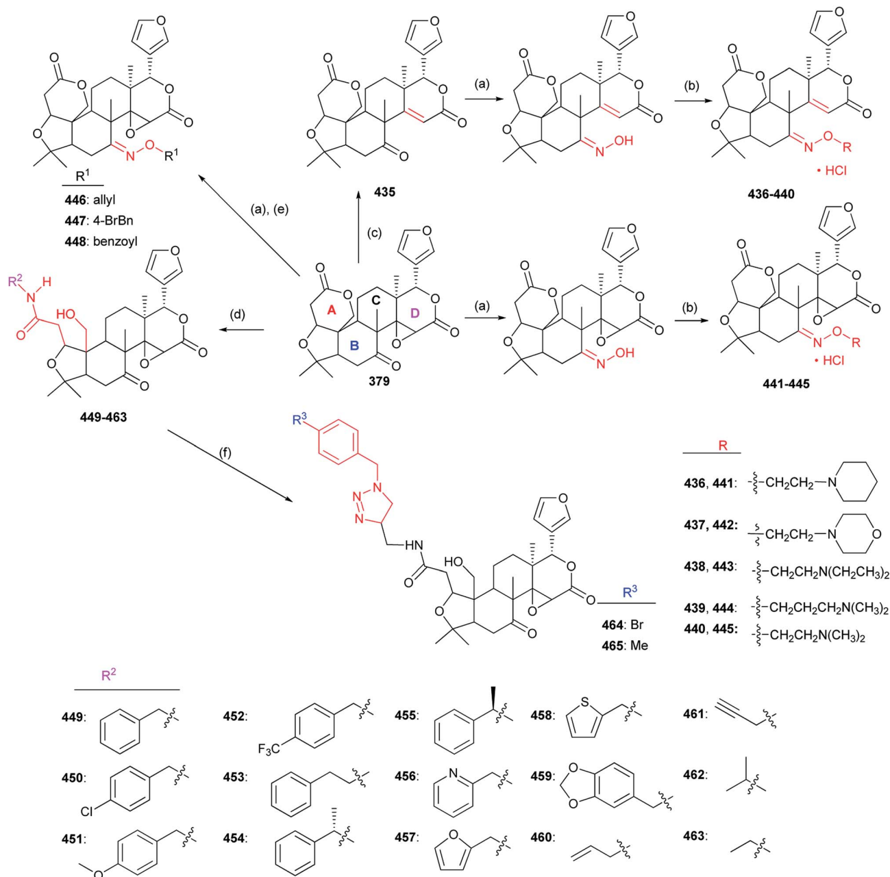
Scheme 7 Semisynthesis of limonin derivatives. Reagents and conditions: (a) \text{NH}_2\text{OH} \cdot \text{HCl} , pyridine, EtOH, reflux; (b) (i) \text{RLi} , NaOH, TBAB, dry THF, 80 °C; (ii) \text{HCl} , dry ether, \text{CH}_2\text{Cl}_2 ; (c) \text{HI} , \text{HOAc} ; (d) condition (i): abs. EtOH, appropriate amine, montmorillonite K-10, microwave-assisted; condition (ii): abs. EtOH, appropriate amine, montmorillonite K-10, reflux; condition (iii): \text{CH}_2\text{Cl}_2 , appropriate amine, montmorillonite K-10, ultrasonic bath; (e) \text{R}^1\text{Br} or \text{R}^1\text{Cl} , NaH, DMF, 0 °C to r.t.; (f) for 461, sodium ascorbate, \text{Cu}(\text{OAc})_2 \cdot \text{H}_2\text{O} , THF : \text{H}_2\text{O} (1 : 1), 1-(azidomethylene)-4-bromobenzene or 1-(azidomethylene)-4-methylbenzene, r.t., 10 h.
