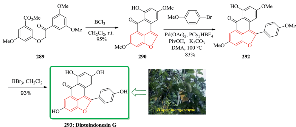
Scheme 63 Total synthesis of diptoinonesin G 293 .
