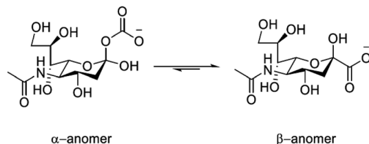
Fig. 1 Structure of sialic acid (Neu-5-Ac) showing the \alpha - and \beta -pyranose forms; \text{pK}_a = 2.6 ( \text{H}_2\text{O} , I = 0.1 , 298 K).
