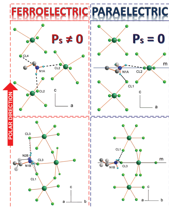
Fig. 3 The details of the cation arrangements in both phases. In paraelectric Phase I, both cations A and B are disordered over the \sigma -m mirror plane with the 0.5/0.5 occupancy ratio; in ferroelectric Phase II, the A moiety is ordered, whereas the B takes two independent spatial orientations with the 0.6/0.4 occupancy ratio at 100 K. Dashed lines stand for hydrogen bonds.
