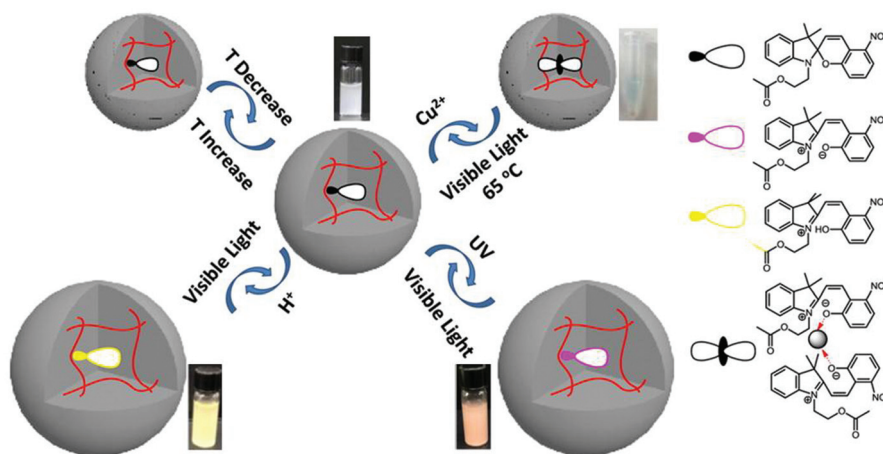
Fig. 8 Spirocyan modified pNIPAm-based microgel response to multiple stimuli. Reprinted with permission from ref. 90. Copyright 2015, American Chemical Society.
