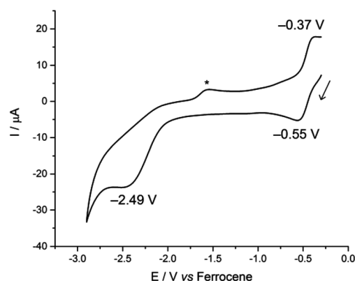
Fig. 3 Cyclic voltammogram of 3 , measured at 100 mV s –1 in 0.1 M CH 2 Cl 2 /[t n Bu 4 N][BPh 4 ]. The asterisk denotes a decomposition product that is formed only after the irreversible reduction.
