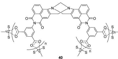
Fig. 21 Structures of the fluorescent chemosensors 39a–c and 40 .
