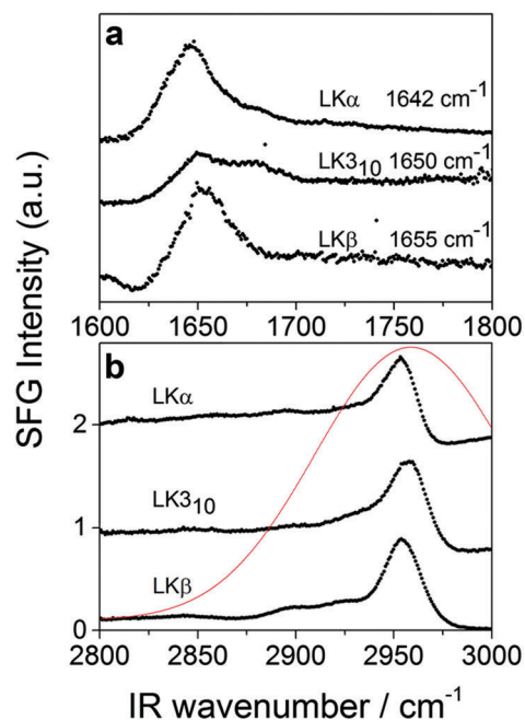
Fig. 1 Static SFG spectra of LK \alpha 14, LK \beta 15, and LK310 adsorbed to the air/ \text{D}_2\text{O} interface (a) amide-I region using ssp polarization (see text for details) (b) using sps polarization combination in the aliphatic stretching region (see text for details). The profile of the excitation pulse is shown in red.
