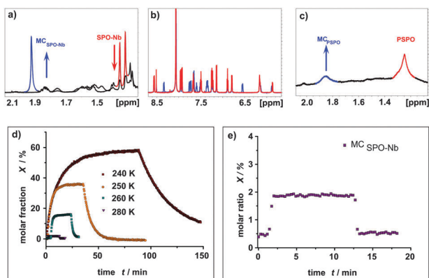
Fig. 5 (a) 1 H-NMR spectra of SPO-Nb solution in DMF-d 7 measured at 240 K prior to (red) and during irradiation (blue) with UV light ( \lambda = 365 nm). (a) Aliphatic region with a severe signal overlap of the two methyl group resonances of the SPO-Nb and resonances of the N -bound aliphatic side chain. (b) Aromatic region with well separated signals for SPO-Nb and MC SPO-Nb . (c) 1 H-NMR spectrum of the PSPO polymer in DMF-d 7 at 240 K during irradiation with UV light with highlighted signals of SPO (red) and MC SPO (blue). (d) Molar fractions of MC SPO-Nb at different temperatures approximated from the integrals of corresponding resonances in a series of 1 H-NMR spectra. (e) Molar fraction of MC SPO-Nb at 280 K.
