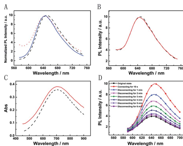
Fig. 5 (A) Emission spectra of 0.1 mg mL -1 Ru@SiO 2 aqueous solution (black dash curve), the Ru@SiO 2 /Nafion electrode (red dot curve) and the PB/Ru@SiO 2 /Nafion film electrode (blue solid curve). (B) Emission spectra of the Ru@SiO 2 /Nafion film electrode before (black dash curve) and after (red solid curve) connecting with Mg. (C) Absorption spectra of the PB (black dash curve) and PB/Ru@SiO 2 /Nafion film electrode (red solid curve). (D) Emission spectra of the PB/Ru@SiO 2 /Nafion film electrode while connecting and disconnecting with Mg.
