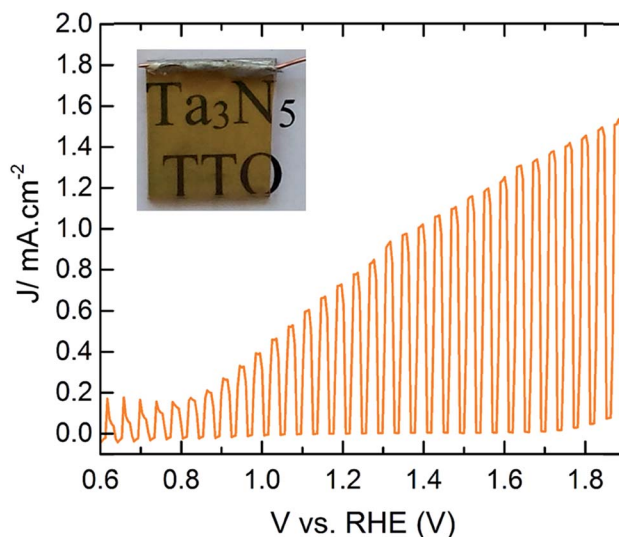
Fig. 5 PEC performance of CoPi modified Ta 3 N 5 (~75 nm) on TTO with 1.6% Ta concentration under 1 sun illumination. The inset is the photograph of the working electrode.
