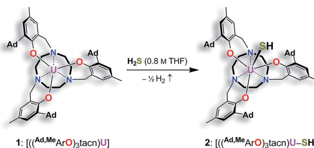
Scheme 1 Synthesis of the uranium(IV) hydrosulfido complex [[(\text{Ad,MeArO})_3\text{tacn}]\text{U-SH}] ( 2 ).
