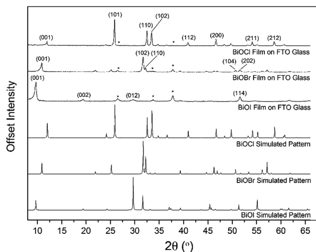
Fig. 3 XRD of BiOX (X = Cl, Br, I) films deposited on FTO glass from the AACVD reaction of \text{BiX}_3/\text{DMF} in air at 300^\circ \text{C} along with simulated BiOX patterns. The asterisked peaks correspond to positions of reflections from the F : SnO (FTO) substrate.
