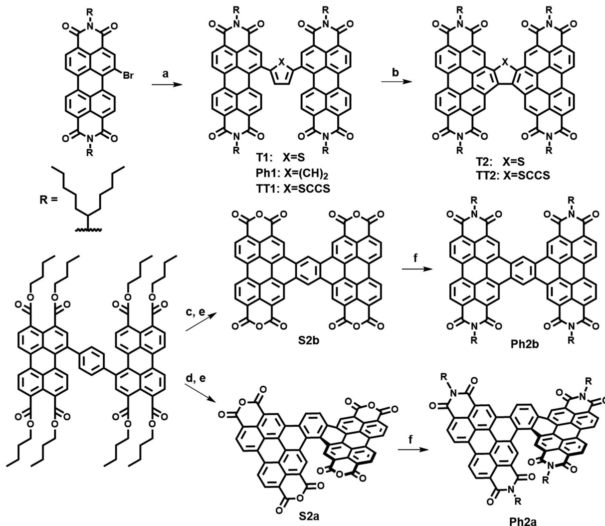
Scheme 1 Synthesis of PDI dimers. (a) Pd(PPh_3)_4 , toluene, (84–90%) (b) h\nu , toluene, air (84–88%) (c) CH_2Cl_2 , I_2 , air, h\nu (d) (1) toluene, I_2 , h\nu , N_2 (2) DDQ (e) ClSO_3H (65–78% over 2 steps) (f) imidazole, 1-pentylhexyl.
