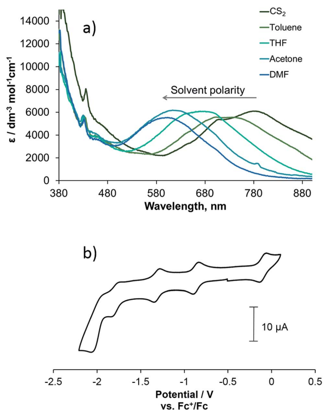
Fig. 1 (a) UV/vis absorption spectra of complex 3 recorded in solvents of different polarity and (b) the cyclic voltammogram of 3 in DMF with [Bu 4 N][BF 4 ] (0.2 M) as supporting electrolyte at a scan rate of 0.1 V s −1 .
