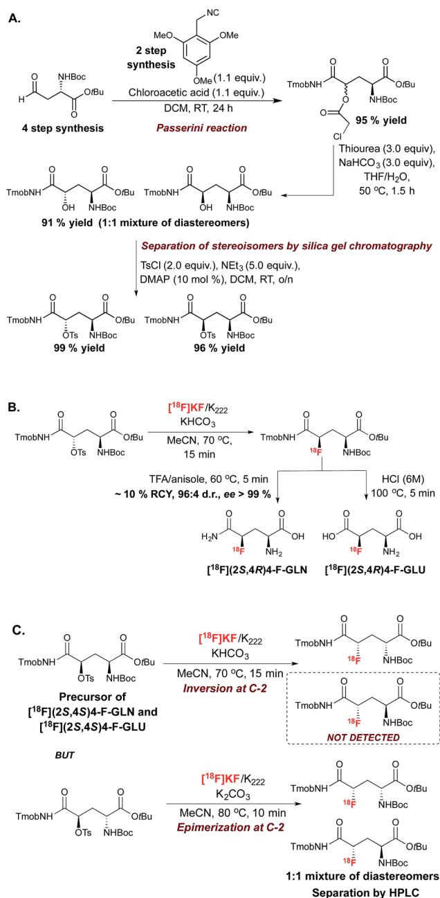
Scheme 2 (A.) Synthesis of the substrates for the radiosynthesis of ^{18}\text{F} 4-F-GLU and ^{18}\text{F} 4-F-GLN. (B.) Radiosynthesis of ^{18}\text{F} -(2 S ,4 R )-4-F-GLU and ^{18}\text{F} -(2 S ,4 R )-4-F-GLN. (C.) Radiosynthesis of ^{18}\text{F} -(2 S ,4 S )-4-F-GLU and ^{18}\text{F} -(2 S ,4 S )-4-F-GLN precursors. Tmob = 2,4,6-trimethoxybenzyl.
