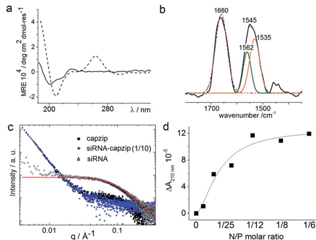
Fig. 3 Capzip folding with and without siRNA. (a) CD spectra for capzip (solid line) and capzip with siRNA (30 \mu\text{M} , dashed line). (b) FT-IR spectra for capzip: raw spectrum (black line), cumulative fit (dotted blue line), deconvoluted amide I spectrum (pink line) and amide II spectra (green and orange lines). Folding conditions: 100 \mu\text{M} peptide, pH 7.4, 10 mM MOPS, 20 ^{\circ}\text{C} . (c) SAXS curves for capzip (200 \mu\text{M} , black), siRNA (20 \mu\text{M} , red) and capzip-siRNA (1/10 N/P molar ratio, blue). (d) Differential absorbance ( \Delta A ) at 210 nm versus N/P molar ratio derived from CD titration spectra for capzip (100 \mu\text{M} ).
