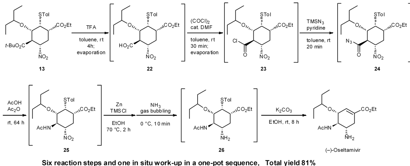
Scheme 2 One-pot synthesis of (-)-oseltamivir from 13.
