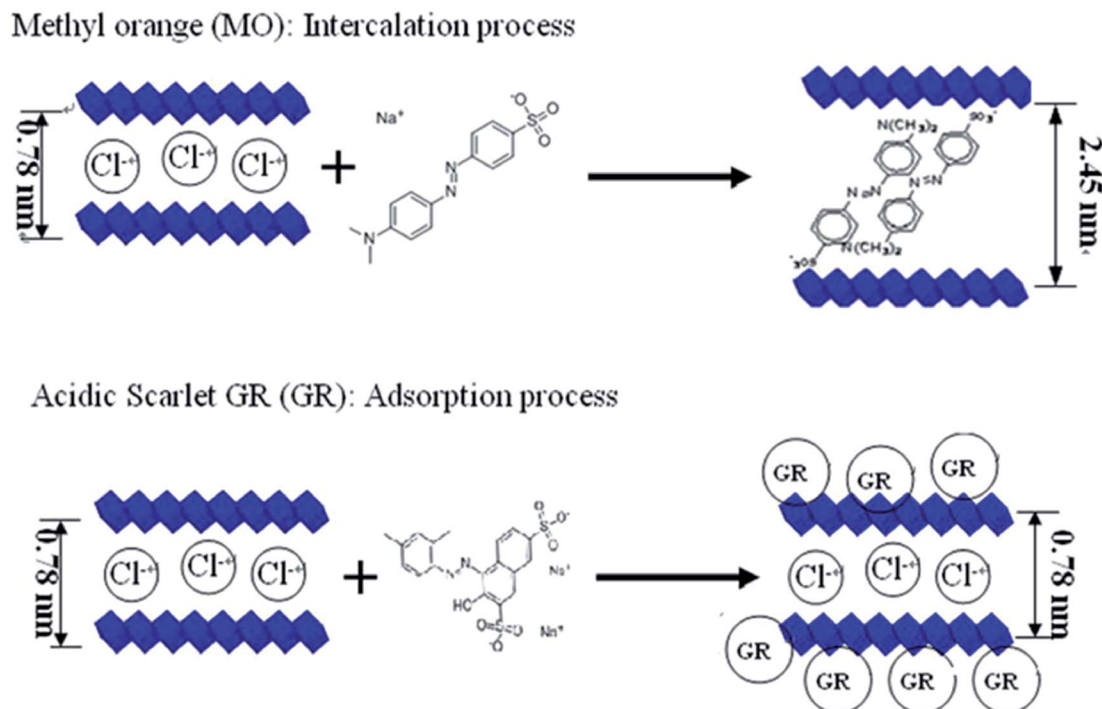
Fig. 10 The models illustration of MO and GR interacted with Ca–Al LDH (adapted from ref. 119 with copyright from 2012 Elsevier).
