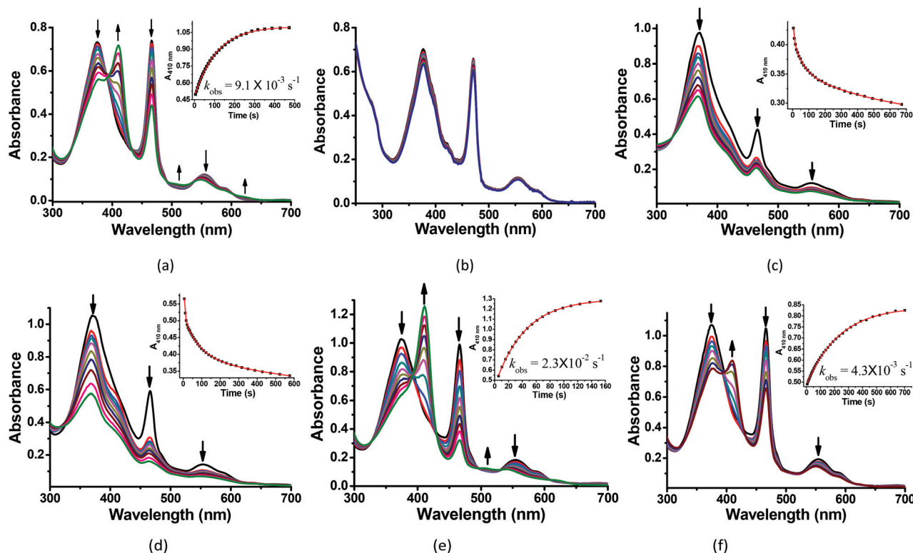
Fig. 2 Kinetic studies of 30 \mu\text{M} (a) His3 Mn III Mb and (b) wild-type Mn III Mb reacted with 200 equiv. KHSO 5 in PBS buffer (pH = 7.4). And 30 \mu\text{M} His3 Mn III Mb reacted with 200 equiv. KHSO 5 at (c) pH = 5.1, (d) pH = 6.0, (e) pH = 7.0, and (f) pH = 8.0. Inset: Time course plots of absorbance at ca. 410 nm, attributing to the formation of the Mn=O intermediate.
