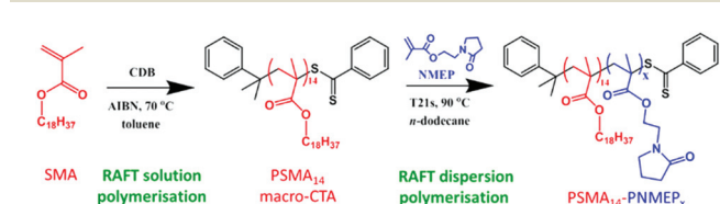
Scheme 1 Synthesis of a PSMA 14 macro-CTA by RAFT solution polymerisation of SMA followed by the preparation of PSMA 14 –PNMEP x nano-objects via RAFT dispersion polymerisation of NMEP in n -dodecane at 90 °C.
