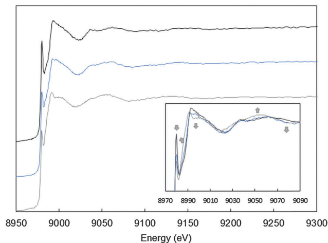
Fig. 3 Cu XANES K-edge X-ray absorption spectra of A\beta_{28} -Cu(I) (black curve), A\beta_{ox} -Cu(I) (blue curve) and A\beta_7 -Cu(I) (grey curve). The conditions were as follows: 0.9 mM Cu(I), 1 mM peptide, and 10 mM dithionite in a HEPES buffer (0.1 M, pH 7.1) solution. Arrows indicate the evolution of the A\beta_{ox} -Cu(I) signature compared with the A\beta_{28} -Cu(I) signature. Inset: zoom of the 8970–9090 eV range.
