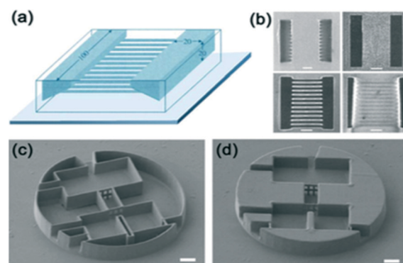
Fig. 16 (a–b) Schematic illustration of a 3D microchannel structure fabricated by two-photon using positive photoresists. Microfluidic structure consists of two rectangular cavities (width, 100\ \mu\text{m} ; length, 20\ \mu\text{m} ; depth, 20\ \mu\text{m} ) and a sloped side wall that are connected by 12 microchannels. (b) Scanning electron micrograph of the final structure, viewed normal to the substrate and two-photon fluorescence images of the final structure at and below the surface. 89 (Copyright 2002 AAAS) (c–d) A conceptual microfluidic device fabricated by 2PP of SU-8. SEM view of the 3D microfluidic systems with 100\ \mu\text{m} diameter disk and 15\ \mu\text{m} height. Here, the internal portion of the background volume is solidified by additional ultraviolet exposure. 90 (Copyright 2009 RSC).
