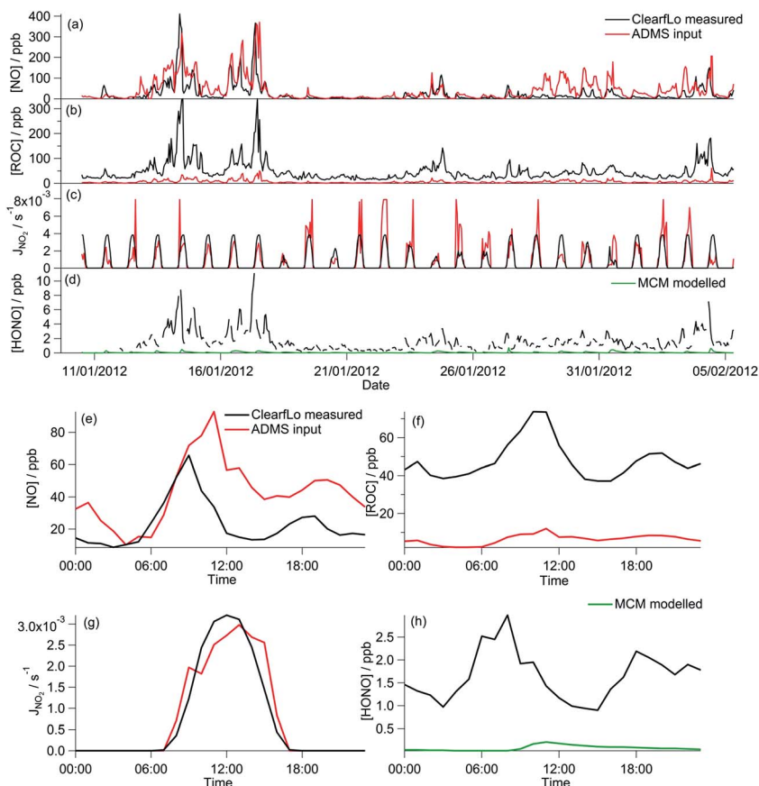
Fig. 8 (a–c) Full time series of ADMS-Urban inputs and measured NO and VOC concentrations and \text{NO}_2 photolysis frequency from ClearfLo winter IOP. (d) Full time series of MCM modelled HONO concentrations and ClearfLo measured HONO. (e–h) Average diurnal cycle of the time series in panels a–d.
