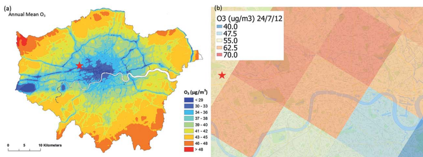
Fig. 1 (a) Contour plot of London showing the annual mean \text{O}_3 concentrations predicted by ADMS-Urban for 2010 constrained to upwind observations. (b) EMEP4UK hourly average surface \text{O}_3 concentrations at 5 km resolution over central London at 12:00, 24/07/2012 (during ClearfLo summer IOP). The star represents the North Kensington site in each case.
