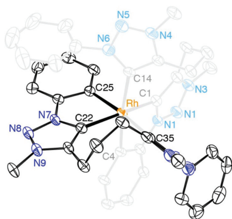
Fig. 5 ORTEP representation of complex 13 (50% probability ellipsoids, \text{Cl}^- counterion, hydrogen atoms, and co-crystallized \text{CH}_2\text{Cl}_2 molecule omitted for clarity); selected bond lengths: Rh–C1 2.041(3) Å, Rh–C14 2.071(3) Å, Rh–C25 2.098(3) Å; selected bond angles: C1–Rh–C4 80.22 (13)°, C1–Rh–C14 91.79(14)°, C4–Rh–C14 171.87(13)°, C1–Rh–C _{\text{trans}} 164.32(13)°.
