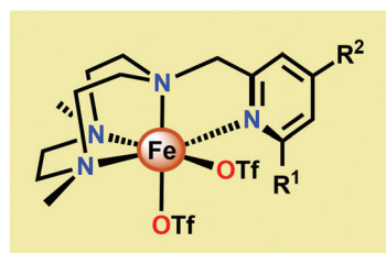
Fig. 28 Fe complexes 54 and 61 – 65 .
