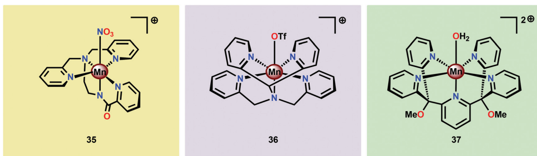
Fig. 18 Structures of mononuclear Mn complexes [Mn(PaPy 3 )(NO 3 )] + (35), [Mn(N4Py)(OTf)] + (36) and Mn(PY5)(OH 2 ) 2 2+ (37).
