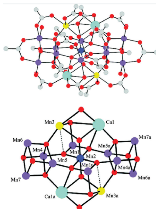
Fig. 19 Structure of the [Mn 13 Ca 2 O 10 (OH) 2 (OMe) 2 (O 2 CPh) 18 (OH 2 ) 4 ] cluster (38) containing [Mn 4 CaO 4 ] sub-units. Color code: cyan (Ca), blue (Mn IV ), violet (Mn III ), yellow (Mn II ), red (O), and grey (C). Reprinted from ref. 141 with permission from the Royal Society of Chemistry.
