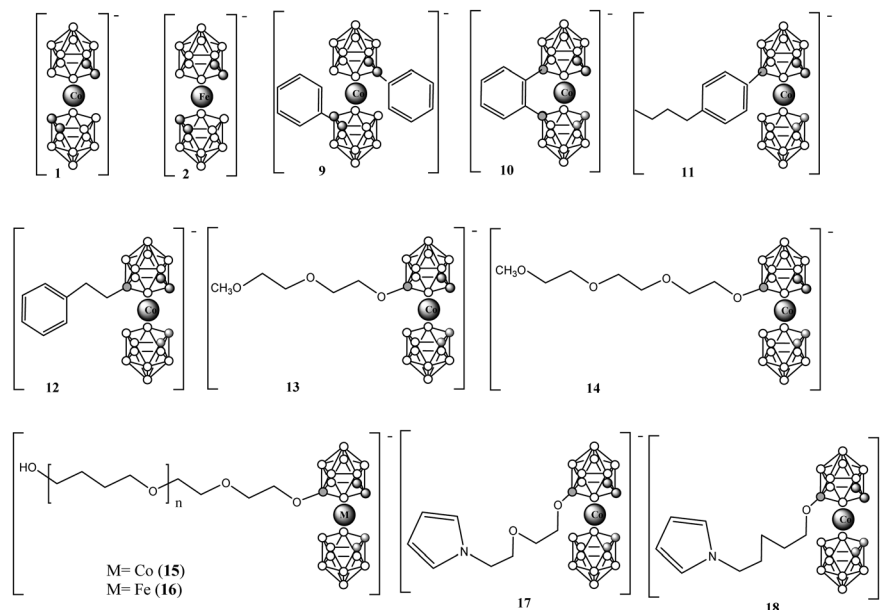
Chart 4 Chemical structures of the anionic metallabisdicarbollides ( 1 ) and ( 2 ) and its derivatives ( 9 )–( 18 ). White circles vertices correspond to B–H while the dark circles to C c –H and grey circle to B atom.
