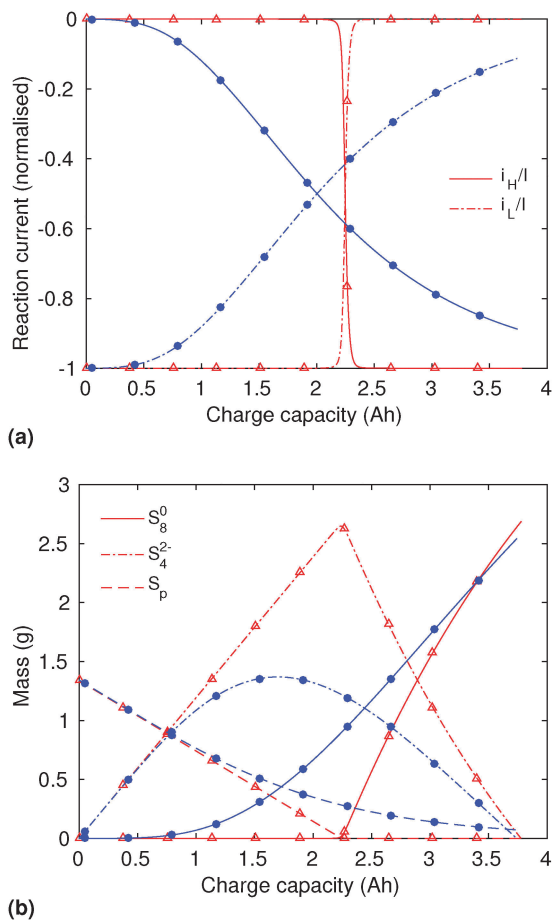
Fig. 4 (a) Simulated reaction currents and (b) species evolution during a 1.7 A ( C/2 ) constant current charge with high saturation concentration S_s^{2-} = 0.005 g, k_p = 100 1/s, (red \Delta ) and low saturation concentration S_s^{2-} = 0.0001 g, k_p = 100 1/s (blue \bullet ). The corresponding voltage is illustrated in Fig. 3(b) with the same symbols. The slower dissolution acts as a bottleneck during charge, triggering an earlier onset of the high plateau reaction and eliminating the boundary between the plateaus. Symbols distinguish between data sets rather than denote computed values.
