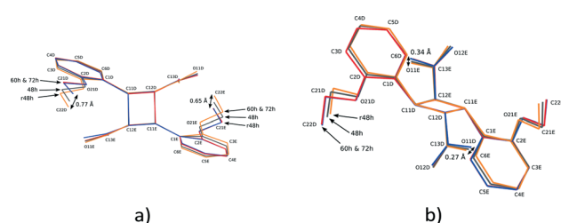
Fig. 8 Two different views of the superimposition of the DE photodimer molecules from the r48 h (final DE product crystal structure after 48 h reaction at 293 K), 48, 60 and 72 h structures.
