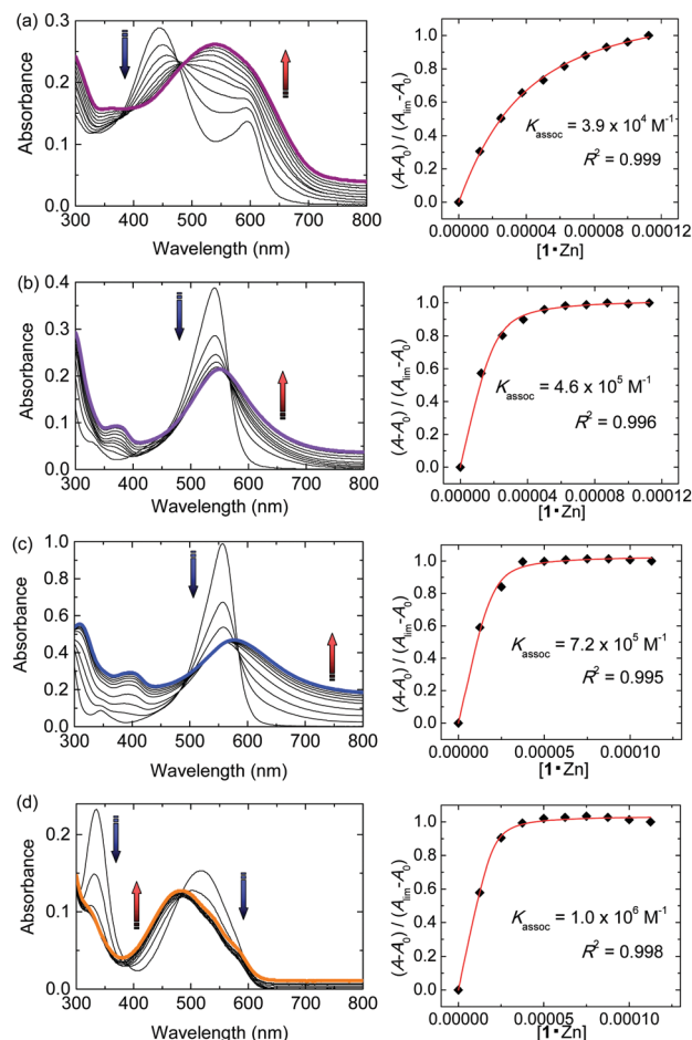
Fig. 2 UV-vis spectra of the diol-dye ( 2.0 \times 10^{-5} M) upon the addition of 1-Zn in HEPES buffer (10 mM) with sodium chloride (10 mM) at 7.5 at 25 °C. [1-Zn] = 0–0.11 mM. (a) PV, (b) PR, (c) BPR and (d) ARS.
