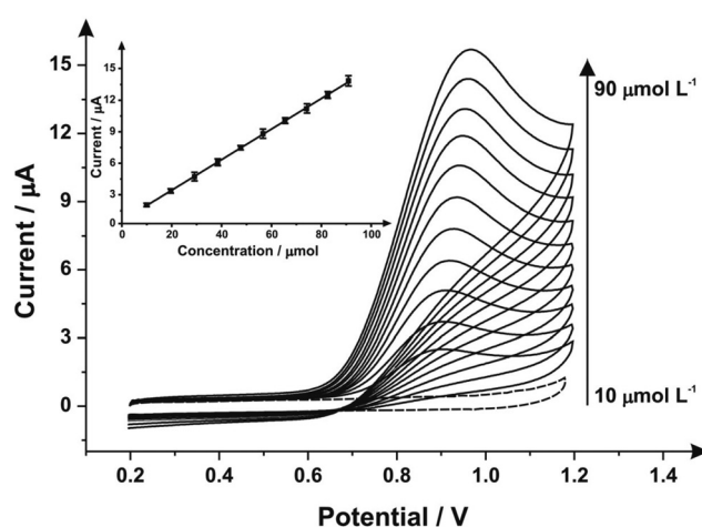
Fig. 4 Cyclic voltammograms obtained from additions of sodium nitrite ( 10\text{--}90 \mu\text{mol L}^{-1} ) into pH 7 PB using a 3 minute mechanical activated/polished SPE with alumina slurry using the same SPE throughout the experimentation (scan rate: 100 \text{ mV s}^{-1} vs. SCE); the dotted line represents the blank (no sodium nitrite) response. Inset: analysis of the voltammetric peak heights as a function of concentration.
