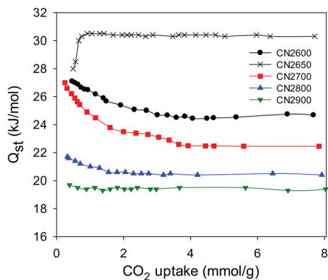
Fig. 10 Isothermic heat of CO 2 adsorption ( Q_{st} ) as a function of CO 2 uptake for activated CN2T samples.
