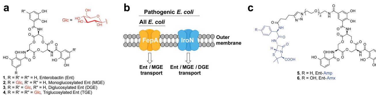
Fig. 1 Siderophores and outer membrane siderophore receptors relevant to this work. (a) Chemical structures of enterobactin 1, and its glucosylated derivatives 2–4. (b) A cartoon representation of the outer membrane receptors FepA and IroN considered in this work. (c) Chemical structures of Ent–Amp/Amx 5 and 6.
