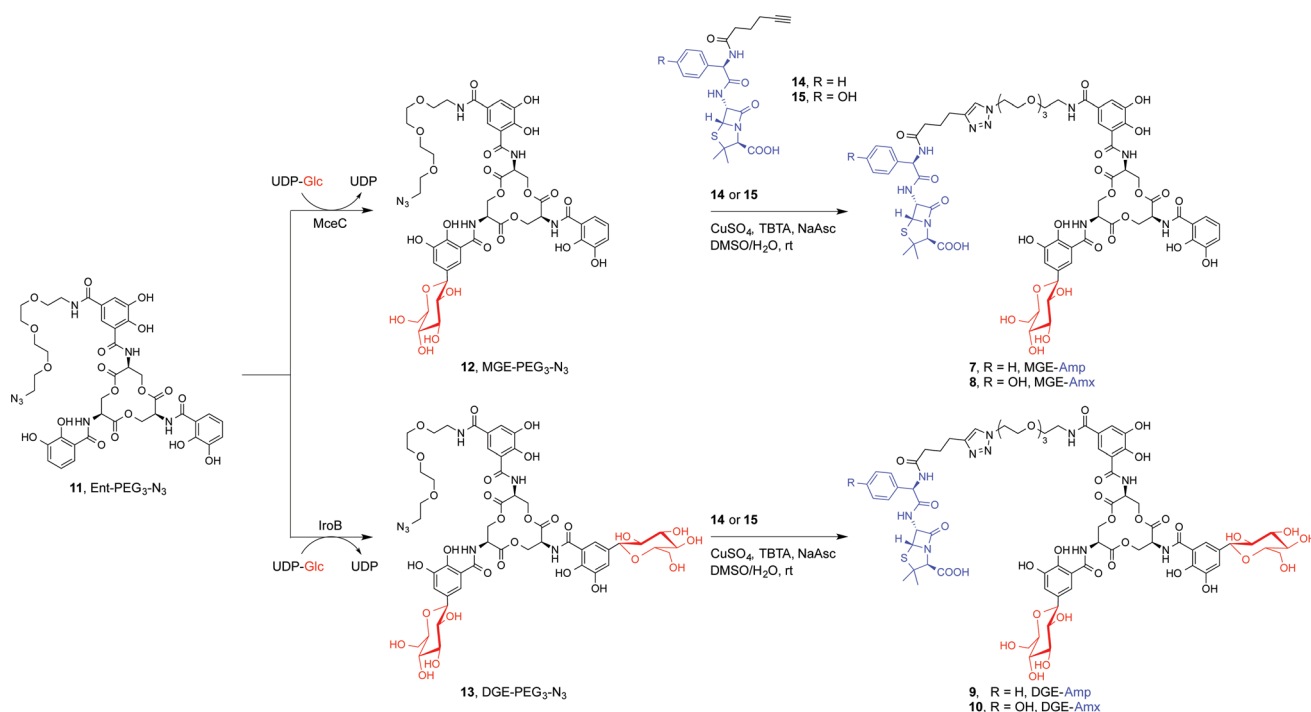
Scheme 1 Chemoenzymatic syntheses of GlcEnt- \beta -lactam conjugates 7–10. The synthetic route consists of MceC- or IroB-catalysed glucosylation of Ent-PEG 3 -N 3 11 followed by a copper-catalysed click reaction to achieve the GlcEnt- \beta -lactam conjugates 7–10. We abbreviate the siderophore family 1–4 (Fig. 1a) as (Glc)Ent and the siderophore- \beta -lactam conjugates 5–10 as (Glc)Ent-Amp/Amx.
