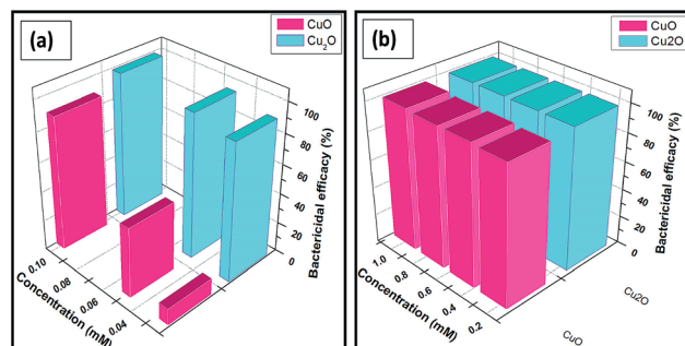
Fig. 3 Detection of bactericidal activity of Trp-CuO and Trp-Cu 2 O nanoparticles at different concentrations ranging from 0.025–0.1 mM (a) and 0.25–1mM (b), suspended in E. coli culture medium for 18 h incubation period.
