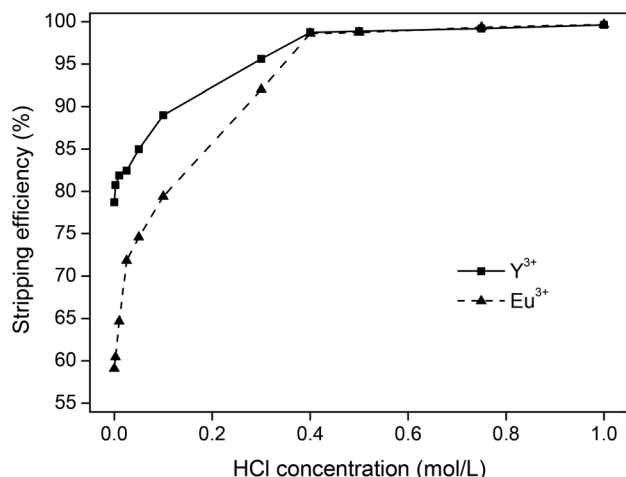
Fig. 7 Stripping of Y 3+ and Eu 3+ from [Hbet][Tf 2 N], previously loaded with 10 mg g -1 of YOX. The influence of the HCl concentration on the stripping efficiency for Y 3+ and Eu 3+ is shown. The biphasic system was shaken (1500 rpm) at 25 °C for 1 h.
