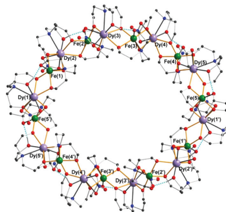
Fig. 1 Structure of the clusters on the example of \text{Fe}_{10}\text{Dy}_{10} : The paramagnetic ions form a ring, which is surrounded by Me-tpa units. The long axes of the elliptical cluster amount to 2.84 and 2.63 nm; the height is 1.27 nm. The inner cavity has dimensions of 1.22 and 0.83 nm, respectively.
