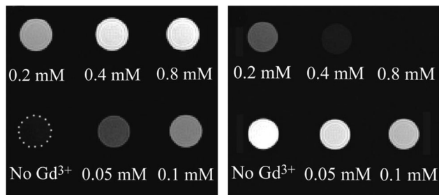
Fig. 29 MR images of \text{NaYF}_4@SiO_2 functionalized with a \text{Gd}^{3+} -coordinating complex with varying gadolinium concentrations (left: T_1 -weighted; right: T_2 -weighted). The reference solution ("No \text{Gd}^{3+} ") contains the \text{NaYF}_4@SiO_2 functionalized with the complex but without any coordinated \text{Gd}^{3+} . The \text{Gd}^{3+} -functionalized UCNPs are more applicable for T_1 -weighted MRI. Reprinted with permission from ref. 147. Copyright © 2009, American Chemical Society.
