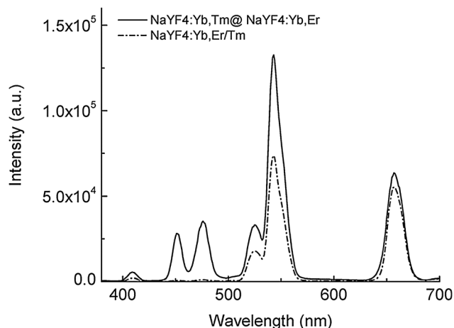
Fig. 5 Luminescence spectra of active-core-active-shell \text{NaYF}_4 UCNP (emission bands of \text{Tm}^{3+} : 409 nm, 450 nm and 475 nm; emission bands of \text{Er}^{3+} : 520 nm, 541 nm and 653 nm). The spatial separation of the two activators in \text{NaYF}_4:\text{Yb},\text{Tm}@\text{NaYF}_4:\text{Yb},\text{Er} avoids quenching of the activators compared to co-doped \text{NaYF}_4:\text{Yb},\text{Er}/\text{Tm} UCNP. Reprinted with permission from ref. 84. Copyright © 2008, American Chemical Society.
