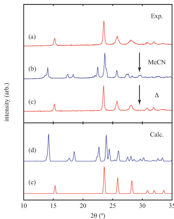
Fig. 7 (Top) Powder X-ray diffraction patterns of (a) as-prepared Cu(tcm), (b) the same sample after exposure to MeCN, and (c) after subsequent heating at 200 °C for 3 h. (Bottom) Calculated X-ray diffraction patterns of (d) [\text{Cu}(\text{MeCN})(\text{tcm})] and (e) Cu(tcm).
