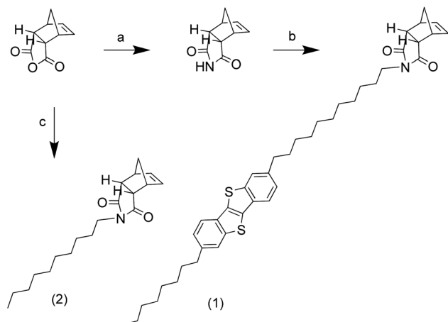
Scheme 2 Synthesis of molecules 1 and 2. (a) 1 eq. \text{NH}_4\text{OAc} , \text{AcOH} , 140^\circ\text{C} , 16 h, 100%. (b) 1 eq. \text{C}_8\text{BTBT-C}_{11}\text{Br} (0.5 g), 1.5 eq. \text{K}_2\text{CO}_3 , 1 : 1 \text{DMF} : \text{THF} , reflux, 16 h, 96%. (c) 1 eq. 1-decylamine, 1 eq. triethylamine, Ar, dry toluene, reflux, 16 h, Dean–Stark app., 86%.
