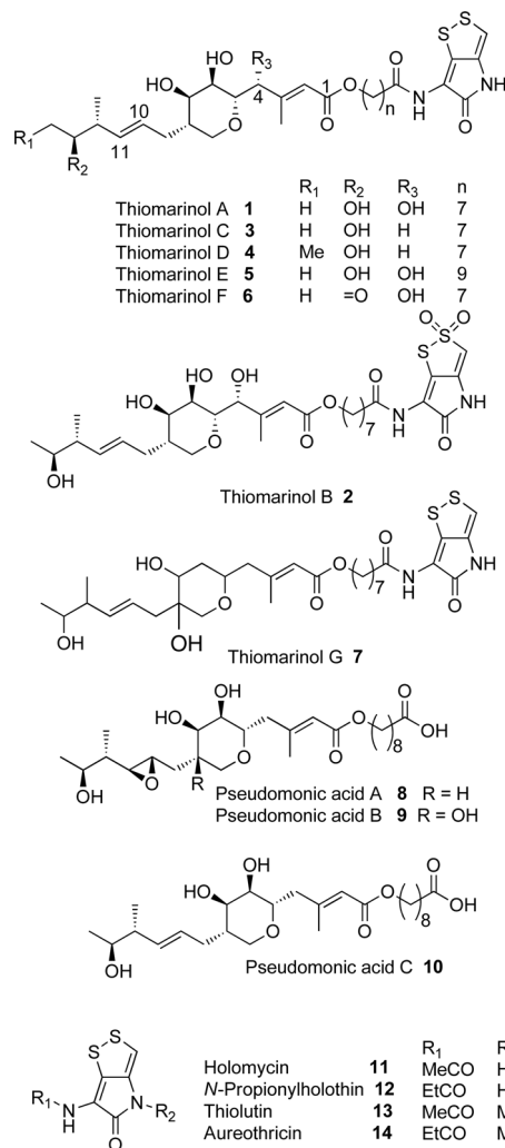
Fig. 1 Thiomarinol, pseudomonic acid and acyl pyrrothine antibiotics.
